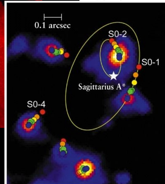
The Centre of the Milky Way (VLT YEPUN + NACO)
